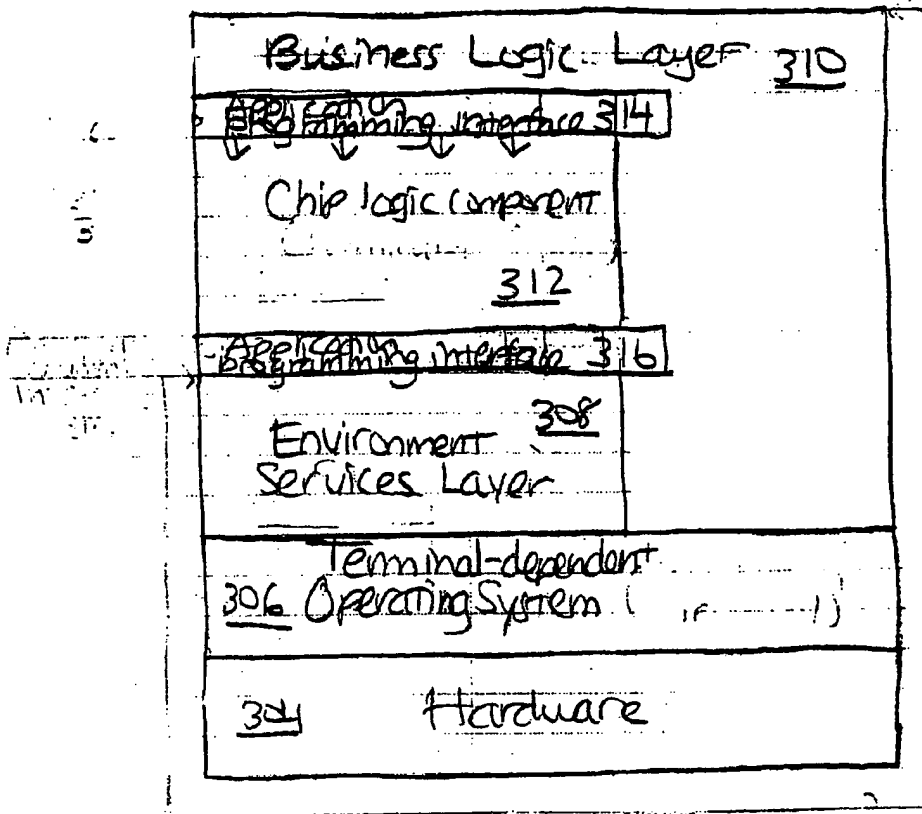
Terminal Software Architecture
